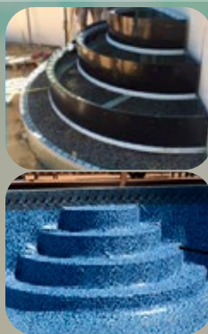
POUR IN PLACE STEP WITH CUSTOM LINER Metal mold filled with crushed stone and sand capped in concrete. Just like a traditional in ground pool!
